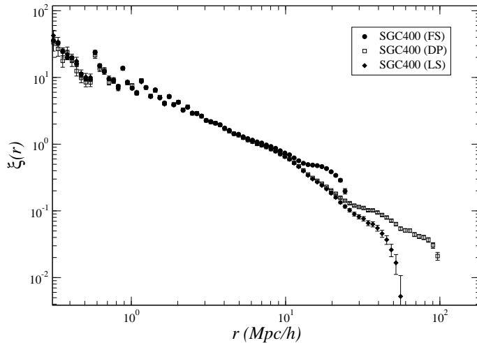
Fig. 21. Standard two-point correlation function in the SGC400 measured by means of different estimators, namely the Full-Shell (FS), the Davis and Peebles (DP) and the Landy and Szalay (LS).
