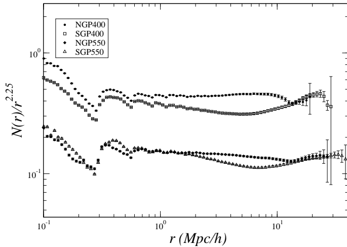
Fig. 13. The same of Fig.12 but divided by the best fit power-law behavior r^{2.25} . The variation of the amplitude B in Eq.12 is more clear in this representation. The determination for r > 20 Mpc/h are subject to systematic fluctuations, due to the limited volume and the weaker statistics.
