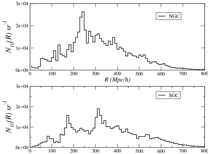
Fig. 18. Upper panel: Radial density in bins of thickness 10 Mpc/h in the NGC magnitude limited sample. The most prominent features identified by the N(r; R) analysis are visible also by the simple counting. There is a large structure at \sim 240 Mpc/h. By comparing this figure with Figs.1-4 one may appreciate the usefulness of the SL method in tracing structures Bottom panel: The same for the SGC magnitude limited sample. Here there are large structures at \sim 180 Mpc/h and \sim 320 Mpc/h.
