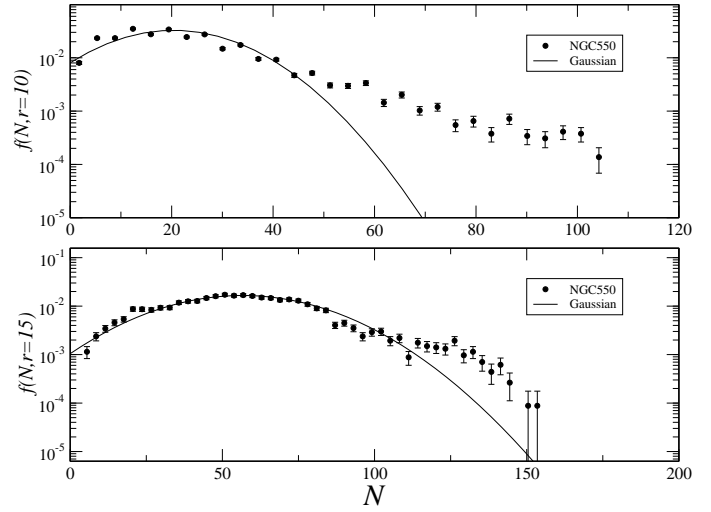
Fig. 8. The same of Fig.7 for the sample NGC550 with r = 10, 15 Mpc/h. For r = 15 Mpc/h there are only 3765 determinations.
