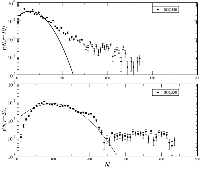
Fig. 10. The same of Fig.7 for the sample SGC550 with r = 10, 20 Mpc/h.
