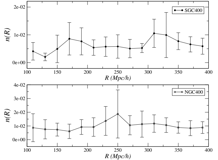
Fig. 16. The average differential radial density \overline{n(R; \Delta R)} (Eq.17) and its error (Eq.18) for the samples NGC400 and SGC400.
