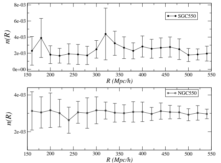
Fig. 17. The same of Fig.16 for SGC550 and NGC550.
