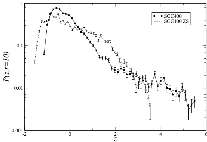
Fig. 28. Comparison between the PDF in the mock sample SGC400m (redshift space) and the one in the real sample SGC400. Poisson error bars are displayed as a reference.
