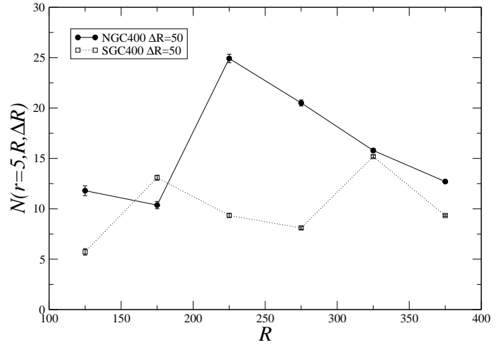
Fig. 14. Behavior of the . Eq.15 with r = 5 Mpc/h for NGC400 and SGC400 and \Delta R = 50 Mpc/h. The error is computed through Eq.16.
