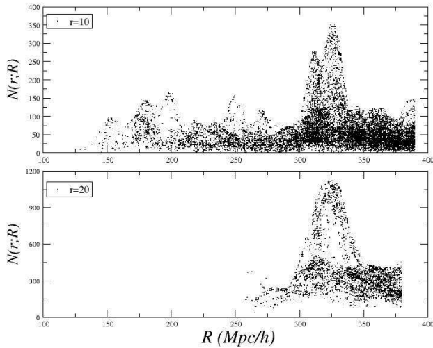
Fig. 3. The same of Fig.1 but now for the sample SGC400 with r = 5, 10, 20 Mpc/h.
