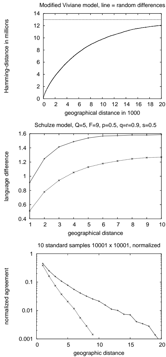
Figure 10: Language differences (in arbitrary units [28]) as a function of geographical distance in the Viviane model (top) and the Schulze model (centre). The horizontal line corresponds to completely uncorrelated languages, that means if all feature values (= bits) were selected randomly. In the central and bottom part, + and x correspond to start with fragmentation (+) and with dominance (x). From [28, 32]. See text for bottom part.
