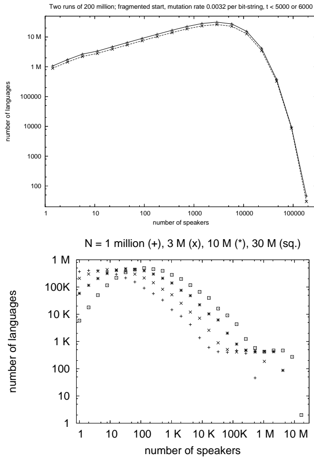
Figure 4: Language size distribution N_s . Top: without lattice, with random multiplicative noise, not in equilibrium [22]. Bottom: On scale-free network in equilibrium [32].
