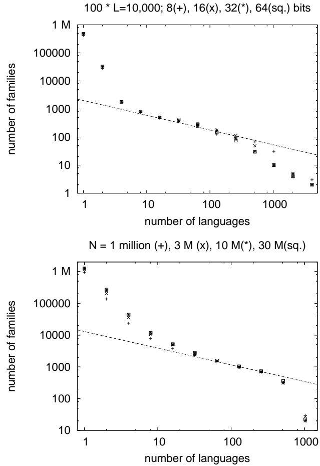
Figure 11: Number of families as a function of the number of different languages in this family [32]. Top: Modified Viviane model for various lengths of the bit-strings. Bottom: Schulze model with Q = 5 , F = 8 on directed Barabási-Albert scale-free network, p = 0.5 , q = 0.59 , r = 0.9 for various population sizes.
