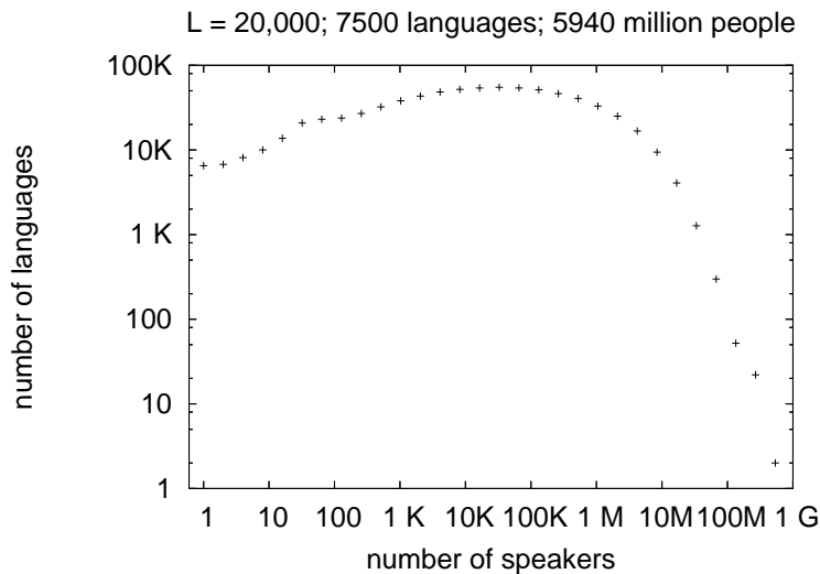
Figure 9: Variation of the number N_s of languages spoken by s people each in the Viviane model, as modified and published in [39].
