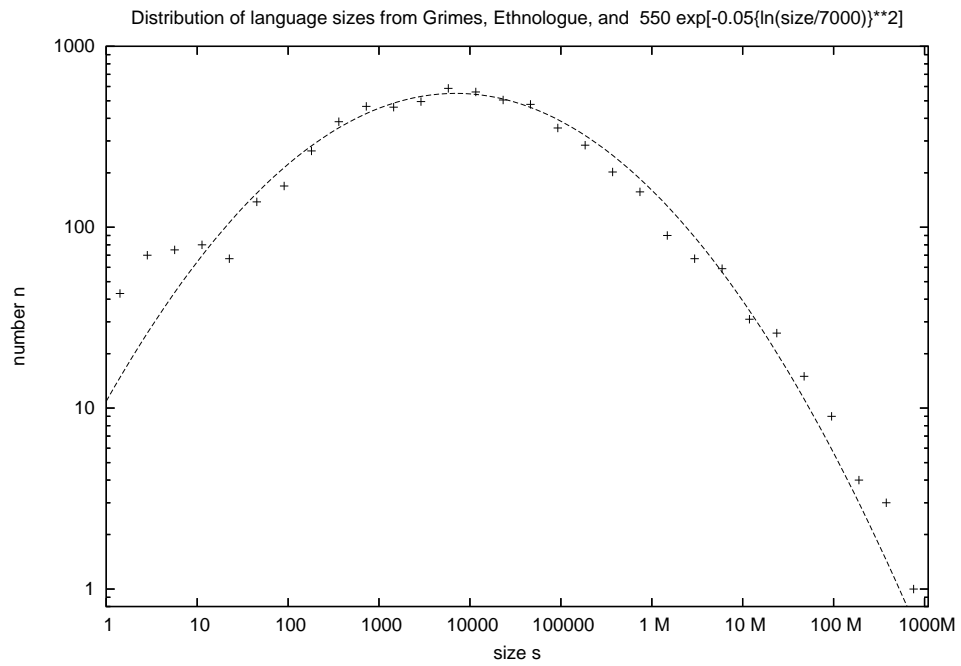
Figure 1: Empirical variation of the number N_s of languages spoken by s people each. For better presentation, the language sizes s are binned in powers of two. Data from Ethnologue [21], as plotted in [22]. The parabola corresponds to a log-normal distribution; we see deviations from it for the smallest sizes [17].
