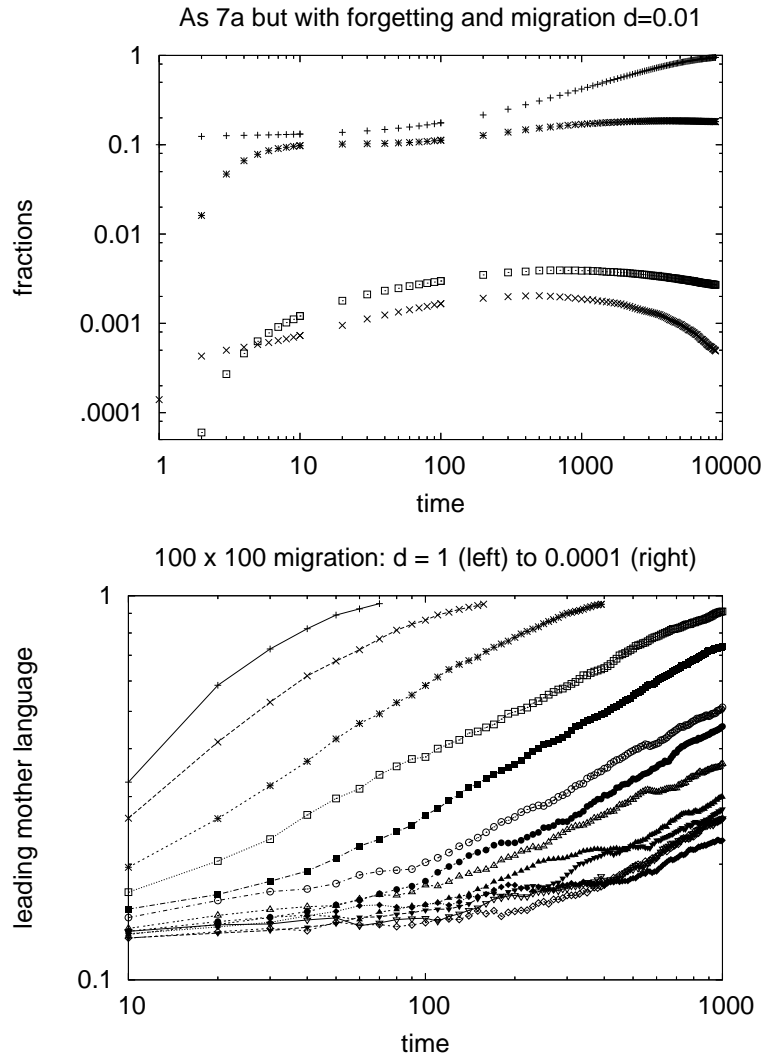
Figure 8: Part a: As Fig 7a, but including a migration probability d of 1 % and a site-dependent forgetting probability between zero and 5 %, on a 6000 \times 6000 lattice. Part b shows the drastic speed-up of dominance if the migration probability d is enhanced: d = 1, 0.5, 0.2, 0.1, \dots, 0.0005, 0.0002, 0.0001 .
