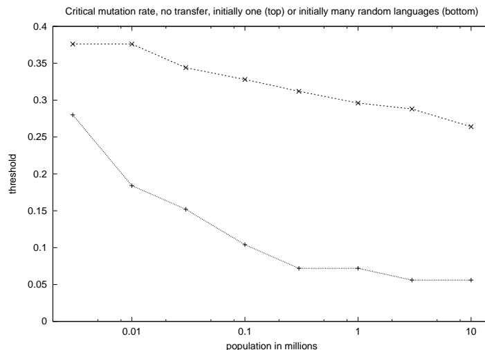
Figure 3: Dependence of the mutation threshold for the phase transition on the population size; upper data from dominance to fragmentation, lower data from fragmentation to dominance. Above the curves we arrive at fragmentation, below at dominance. From [11].
