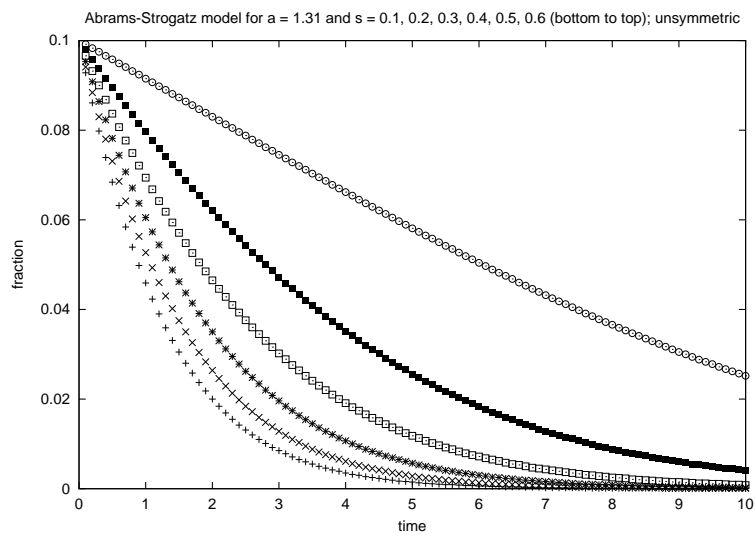
Figure 13: Abrams-Strogatz model: Fraction of people speaking language X, versus time, for an initial concentration of only ten percent and various prestige values s of this language. For s \geq 0.7 this language finally wins over the other language Y. From [3].
