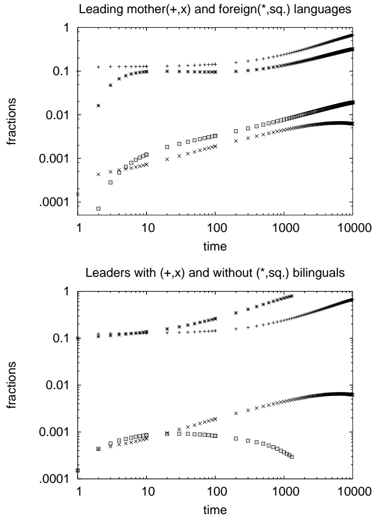
Figure 7: Largest and second-largest languages in the Schulze lattice at p = 0.01 , q = r = 0.9 in a 8000 \times 8000 lattice without migration. Part a includes bilinguals, part b compares only the mother languages with and without bilinguals.
